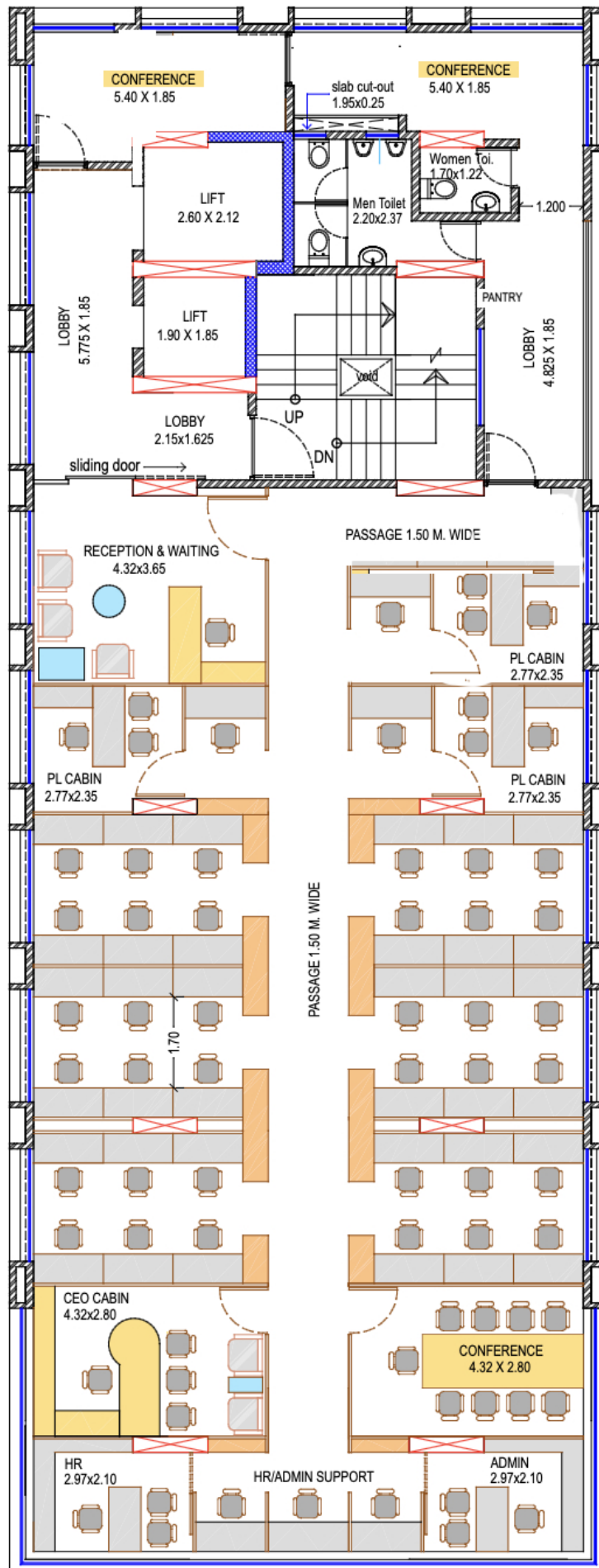
TYPICAL FLOOR PLAN (FIRST TO SEVENTH FLOOR)
